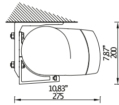
Ceiling installation
