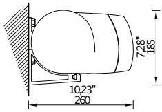
Wall installation
